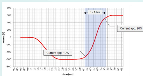
▲ The above testing figures are obtained using PBT 1000 800V/600A System
